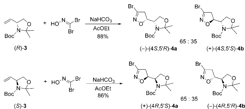
Scheme 2. Synthesis of the Target Amino Acids
