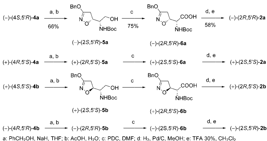
Scheme 2. Synthesis of the Target Amino Acids
