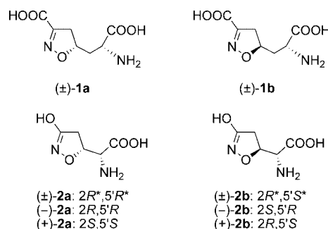
Figure 1. Structures of reference [(±)-1a, (±)-1b, (±)-2a, and (±)-2b] and target compounds [(-)-2a, (+)-2a, (-)-2b, and (+)-2b].
